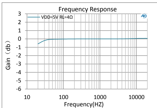
图6: Frequency Response
