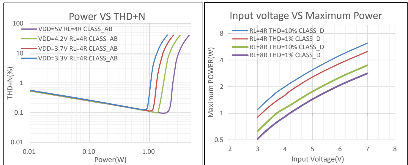
3、Power VS THD+N%
