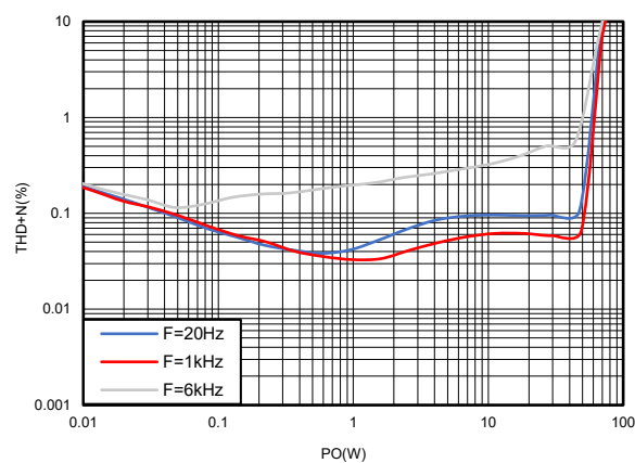
图29. 24V供电8Ω负载THD+N曲线PBTl
